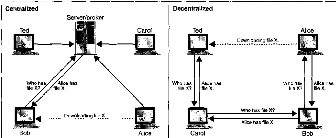
Figure 4: Peer-to-Peer Models
